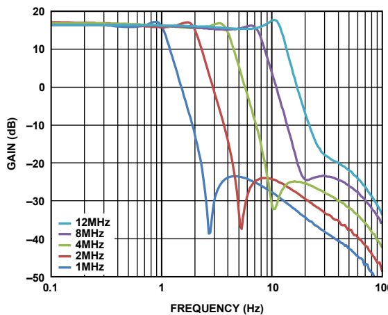
Figure 14. Filter Response
